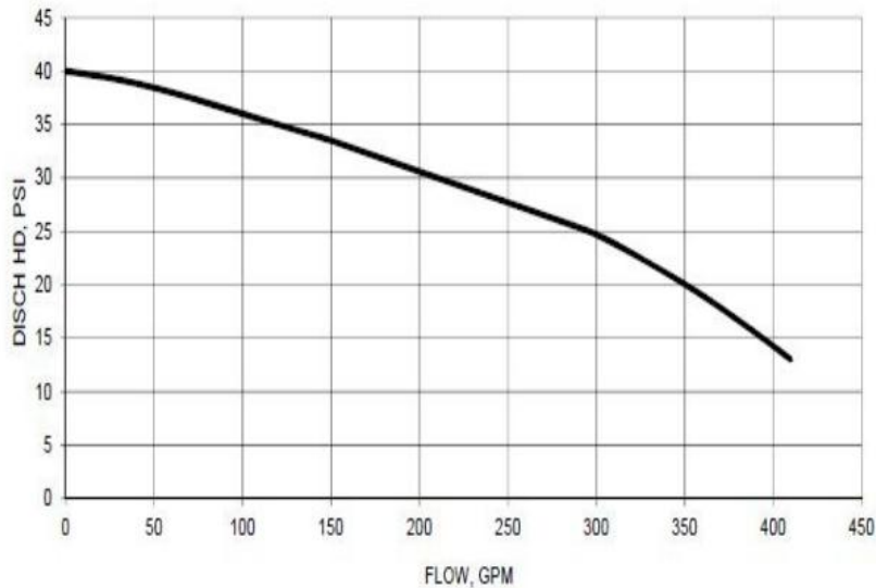
Performance Curve for 3" Trash Pump PU0330
